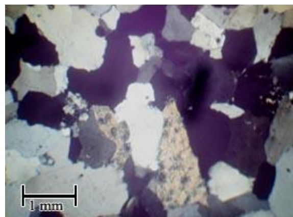
Figure 18: Chlorite as an Authigenic Mineral
