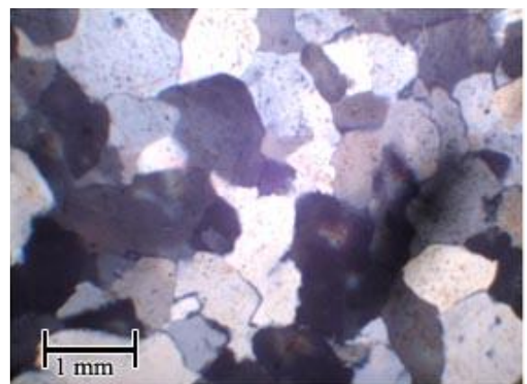
Figure 6: Micro-Stylolitic Contacts
