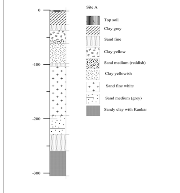
Figure 4: Litholog of a Tubewell at Kolaghat Block, Tamluk Subdivision
