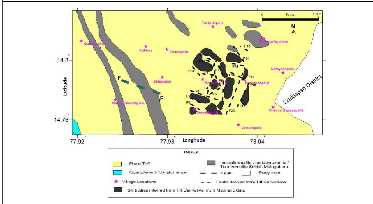
Figure 3: Structural Map inferred from Tilt Derivative Technique
